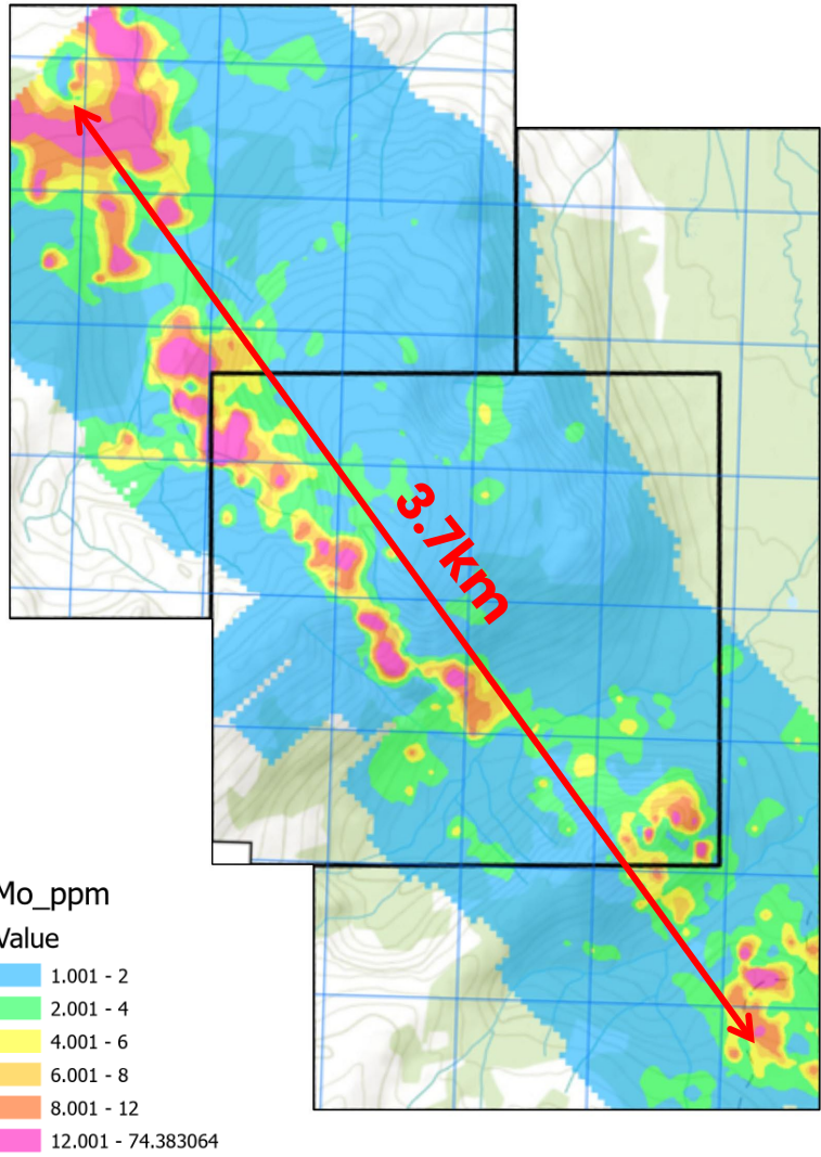
Molybdenum in soil
