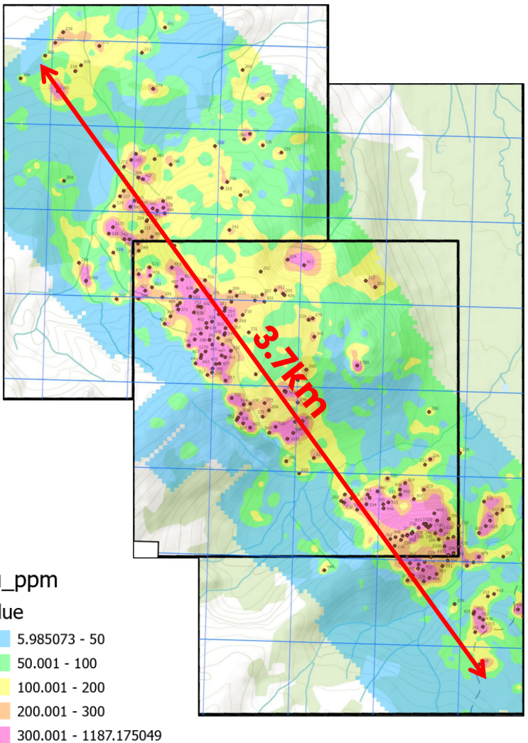
Copper in soil
