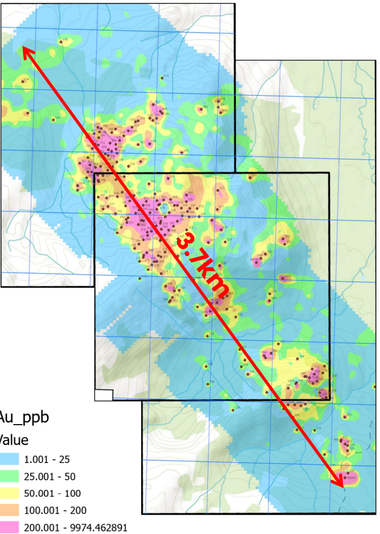
Gold in soil
