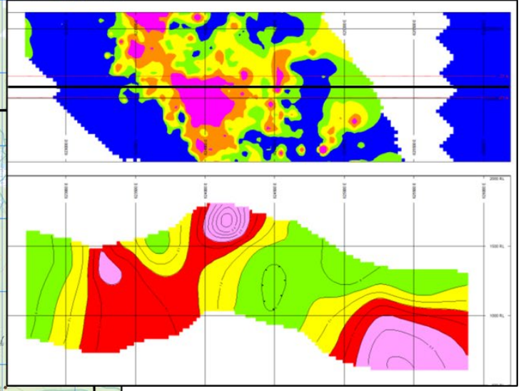
3D IP Inversion
