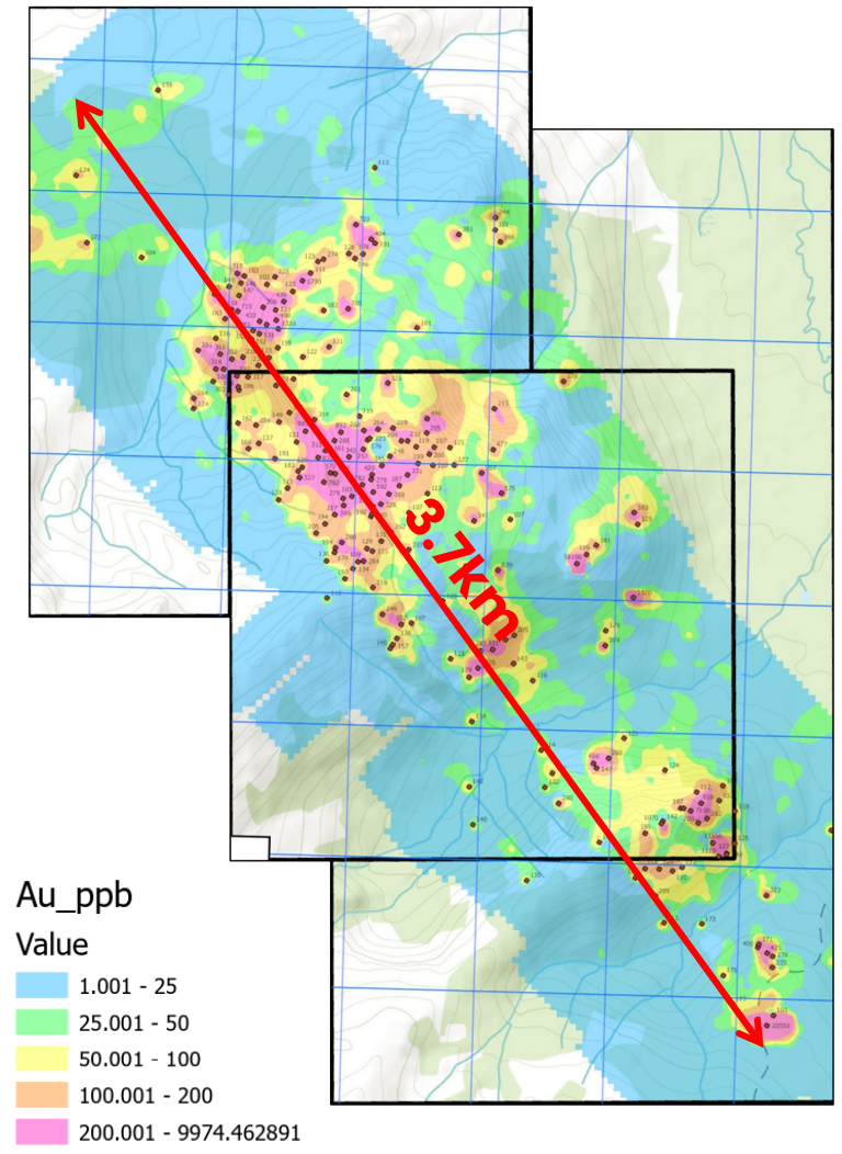
Gold in soil
