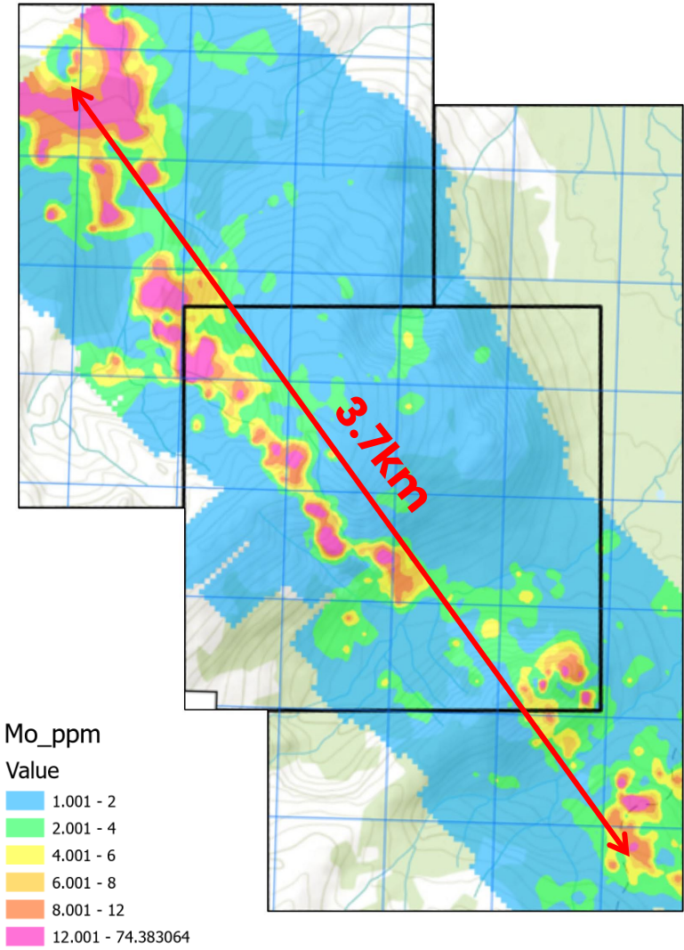
Molybdenum in soil
