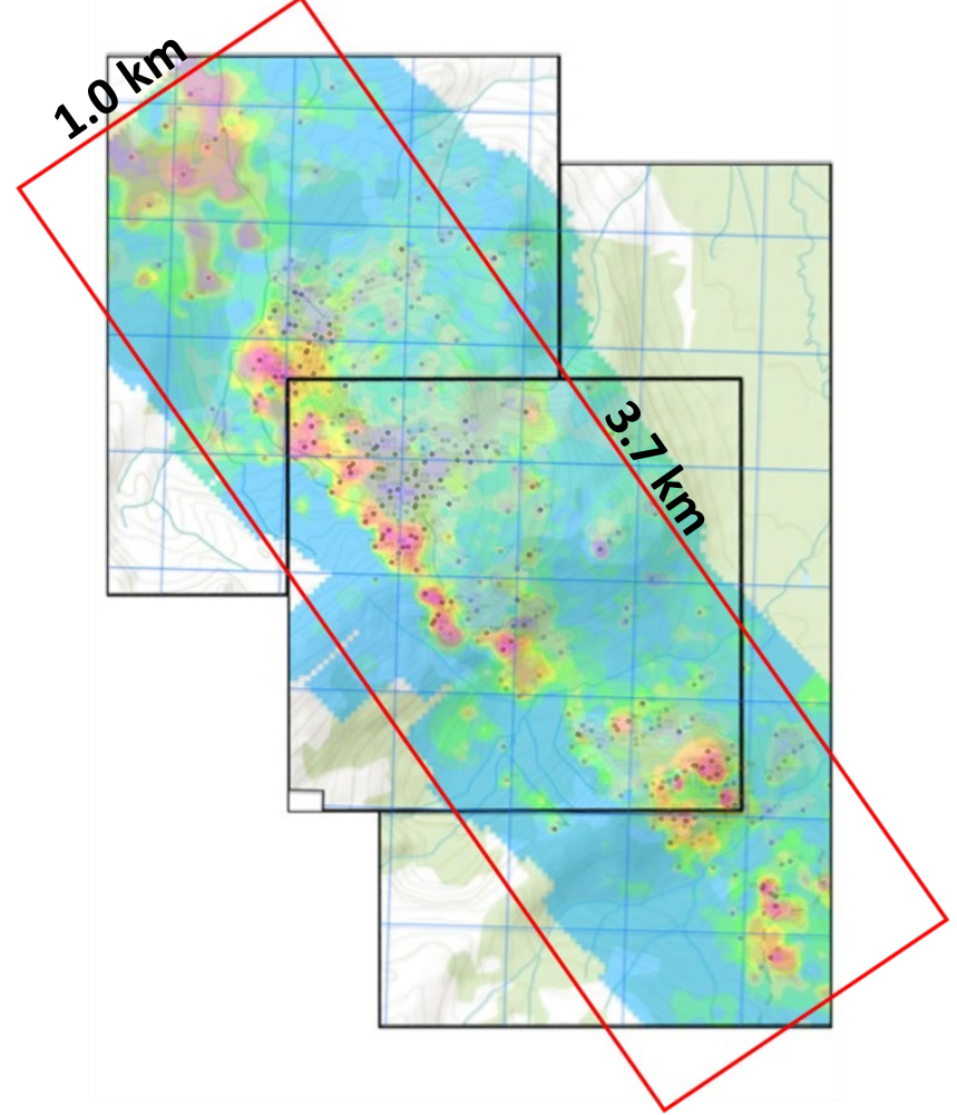
Coincident Au, Cu & Mo Soil Geochemistry
