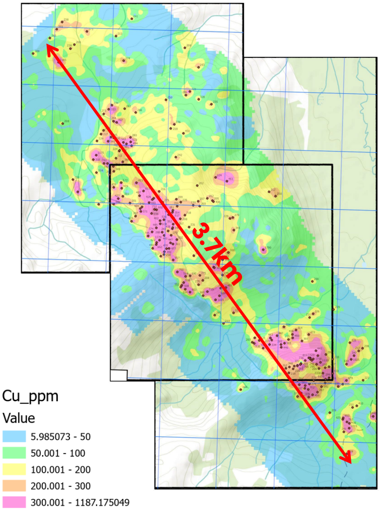
Copper in soil
