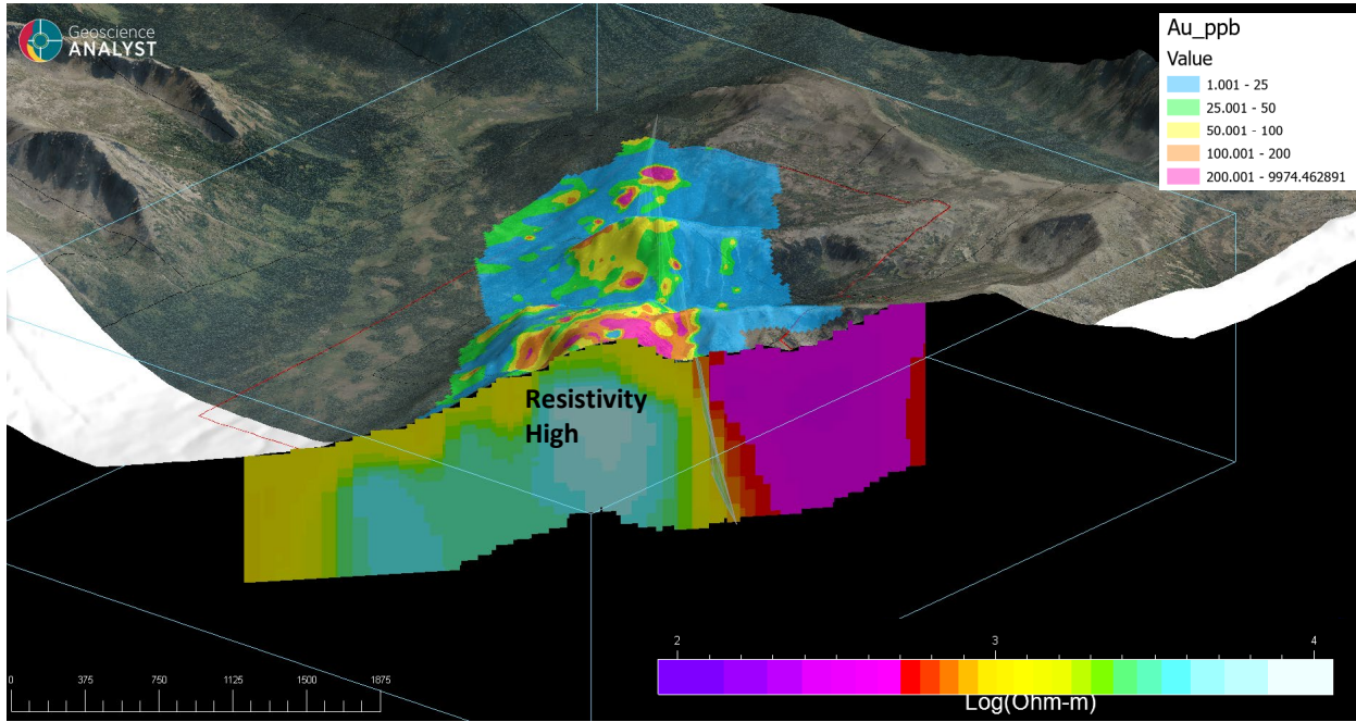
3D Modelled Resistivity (ohm-m) with draped Gold in Soil Geochemistry View to SE
