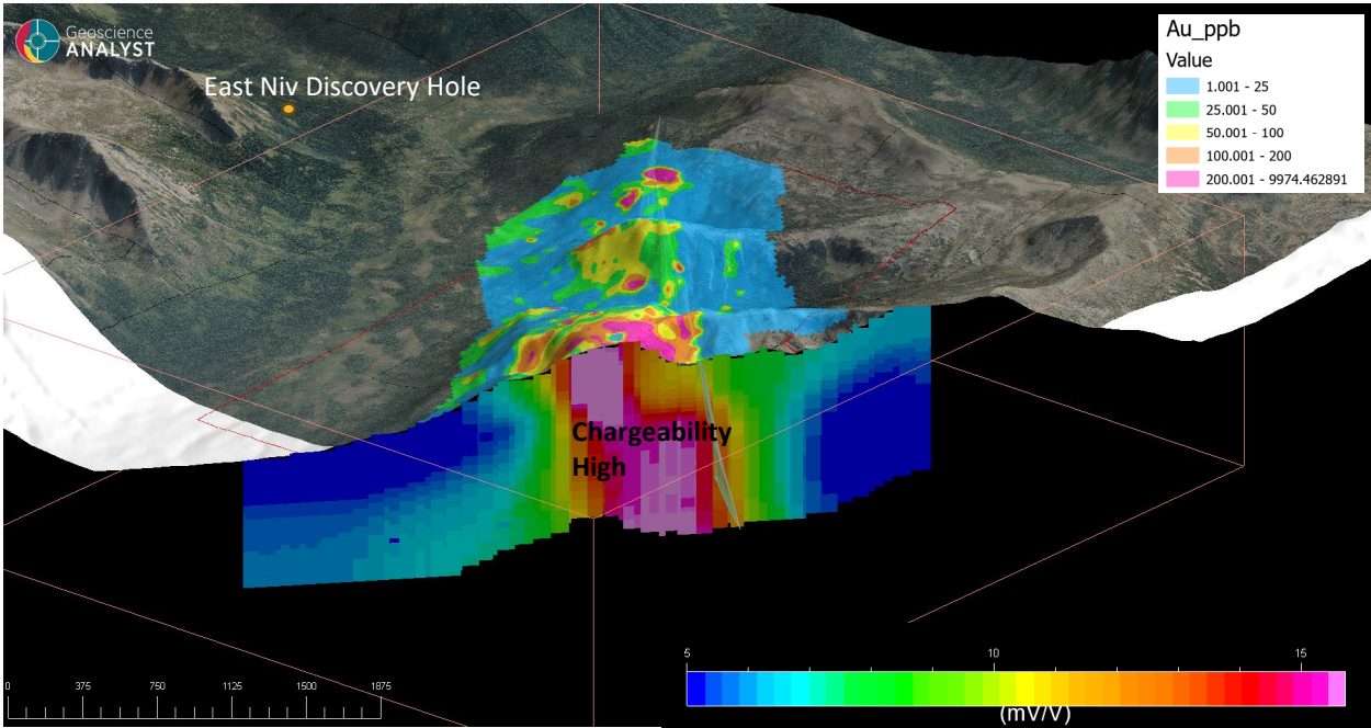
3D Modelled Chargeability (mV/V) with draped Gold in Soil Geochemistry View to SE
