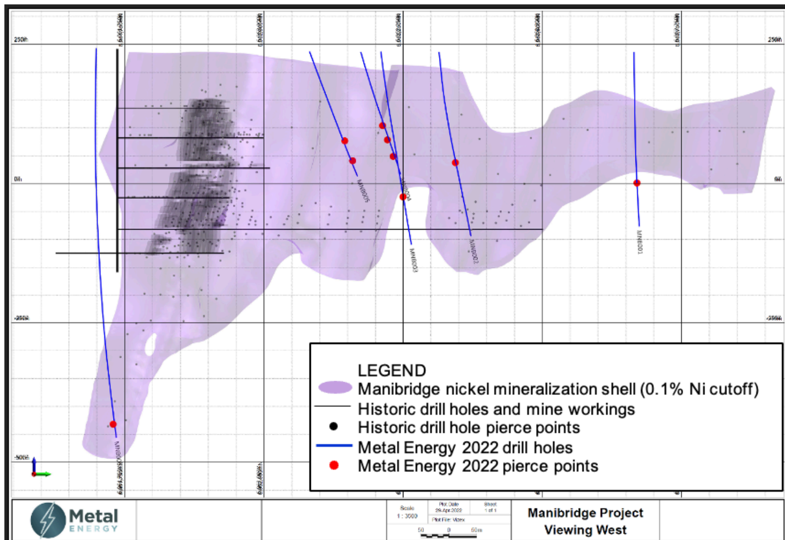
FIGURE 2 – Winter 2022 Drill Holes Within Manibridge Mineralization Shell (looking west)
